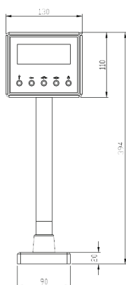
Scale Indicator Front View
