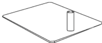
Metal plate for EE-750R Metal plate for stand EE-750 Color: Grey Width: 160 mm Length: 200 mm Material: Platemetal Can be used in combination with 'Holder EE-750R for Stand (14521) and Tube 12mm for metal plate (14524).'
