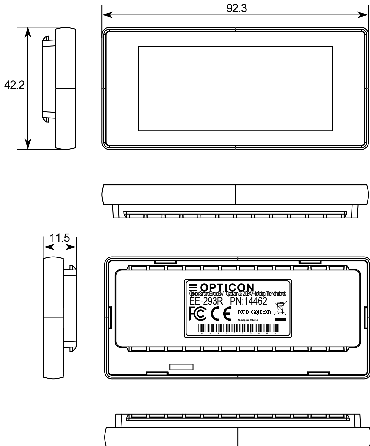
Figure 8: Mechanical drawing
