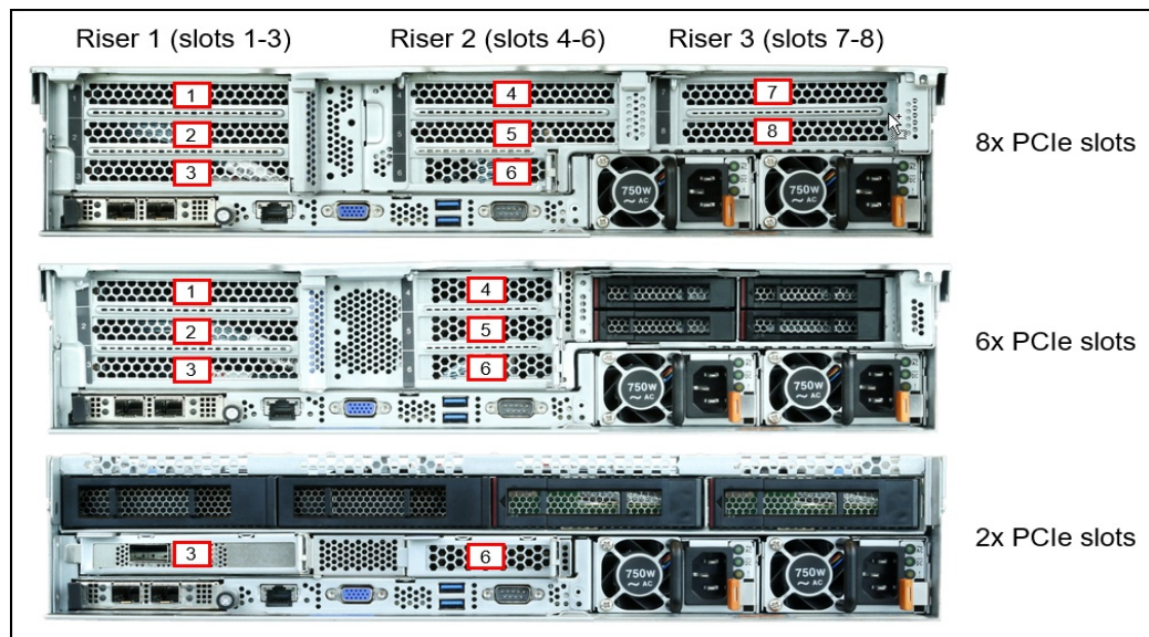
Figure 10. SR655 slots
