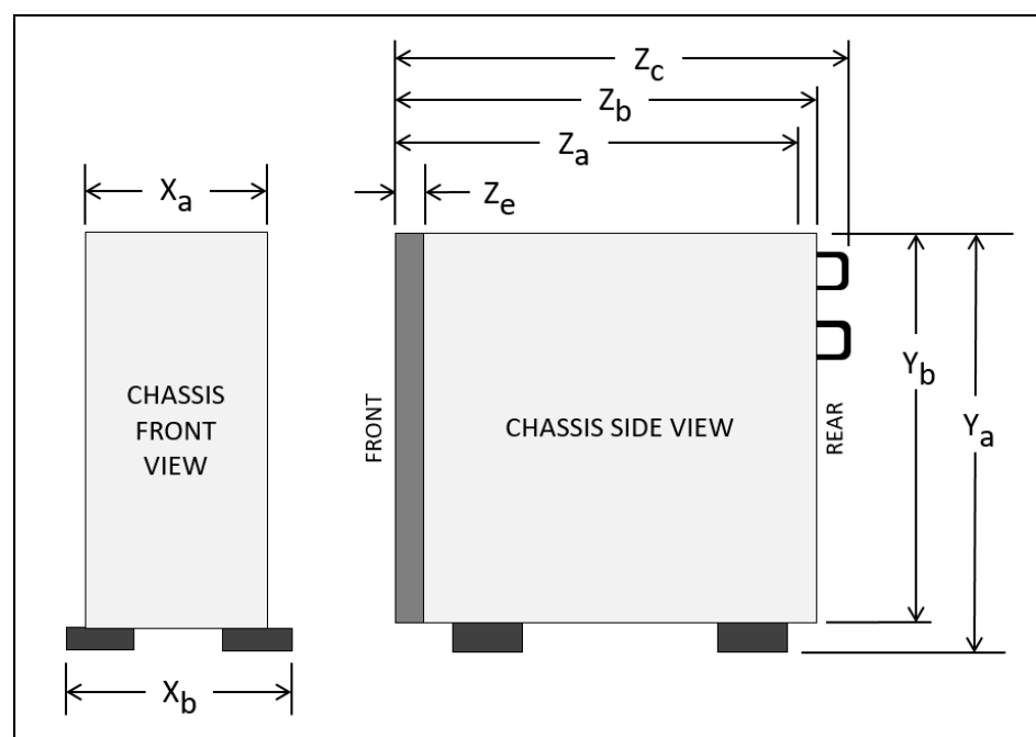
Figure 9. Server dimension
