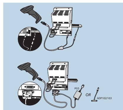
Keyboard Wedge and RS-232 connection
