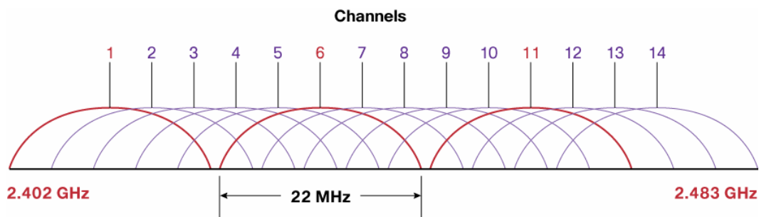
Figure 9. IEEE 802.11b/g DSSS Channel Allocations
