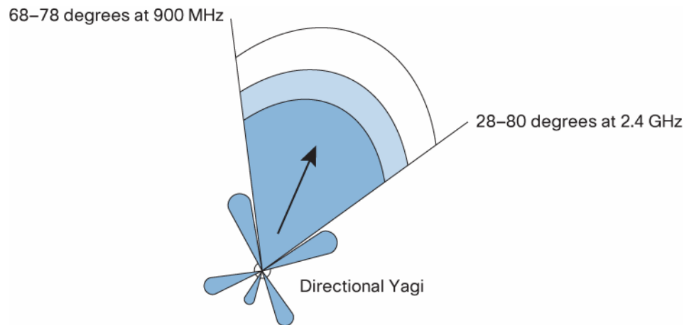
Figure 3. YAGI Antenna
