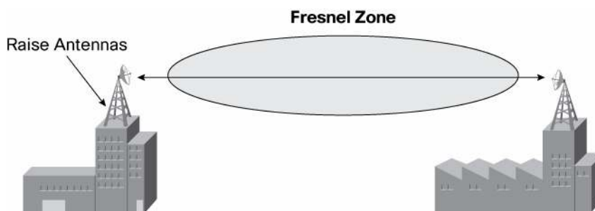
Figure 6. Fresnel Zone
